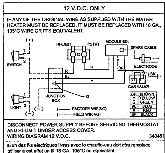
Wiring Diagram 12 V.D.C.
